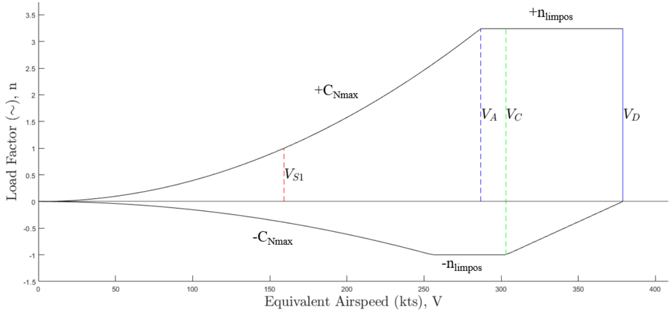
Figure 9.0.3 Maneuvering Diagram
