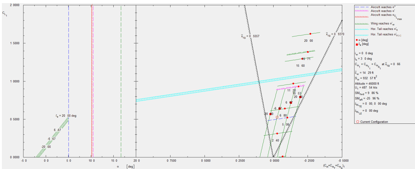
Figure 17.0.1 AETHER Trim Diagram During Cruise
