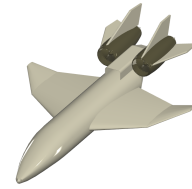
Figure 8.1.11 Twin V-Tail
