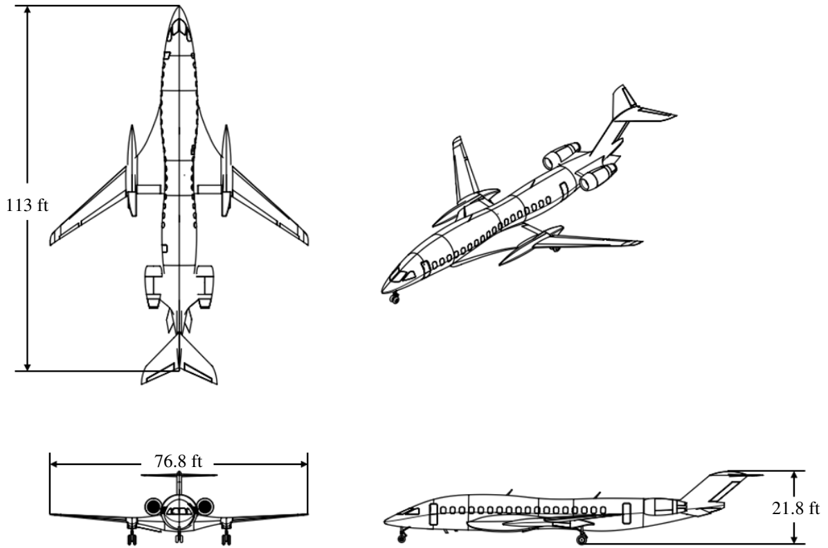
Figure 13.0.1 AETHER Three-View
