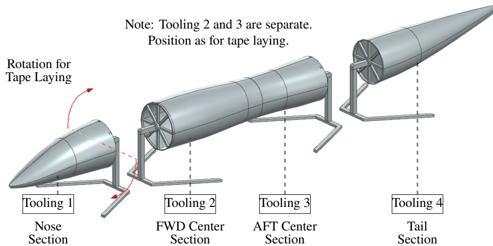
Figure 14.2.1 Fuselage Tooling
