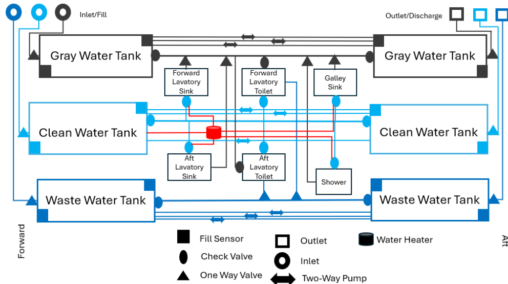
Figure 15.14.3 Water and Waste System
