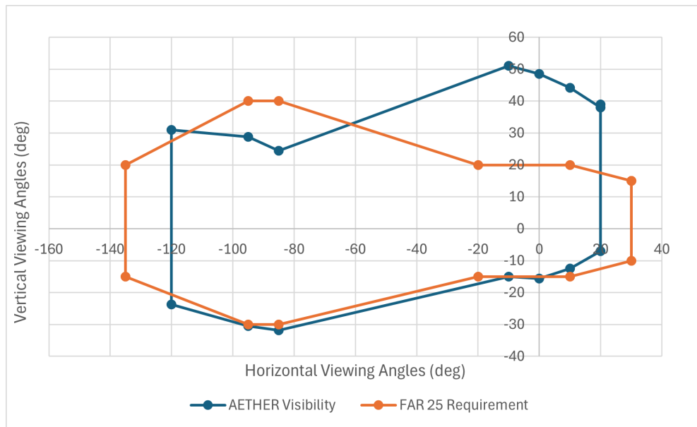
Figure 11.1.3 Pilot Visibility Chart
