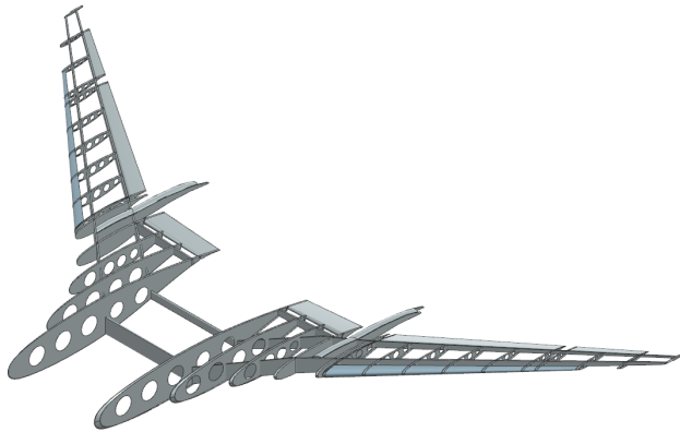
Figure 13.2.3 Wing Substructure
